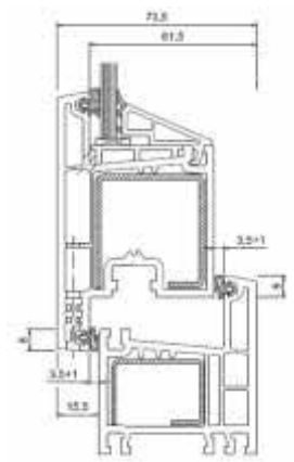
Sectional Details
