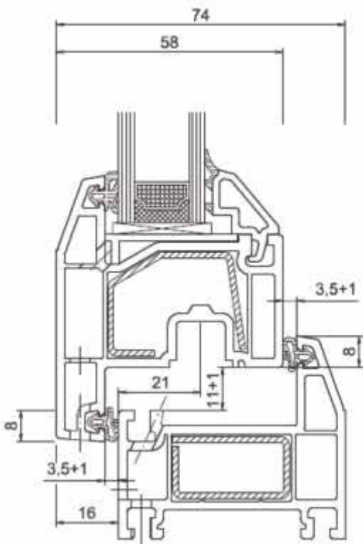
Sectional Details
